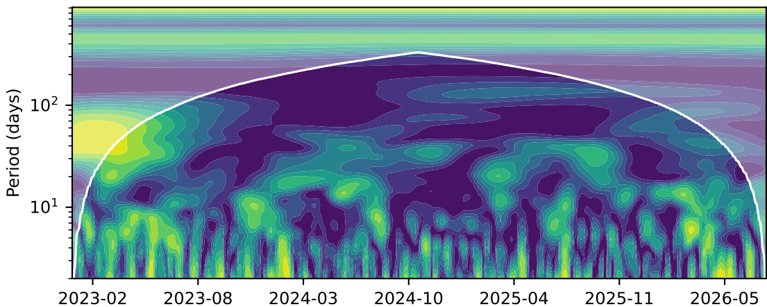
IEF vs. GLD: wavelet coherence
