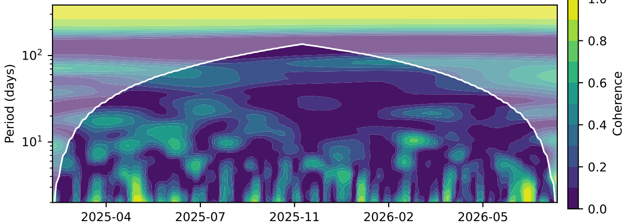
IEF vs. GLD: wavelet coherence
