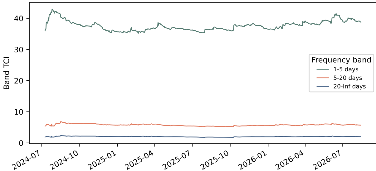
Baruník-Křehlík frequency-domain connectedness
