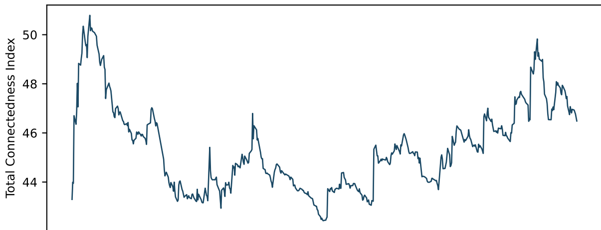
TVP-VAR time-domain connectedness (System R1, \kappa=0.99/0.99 )
