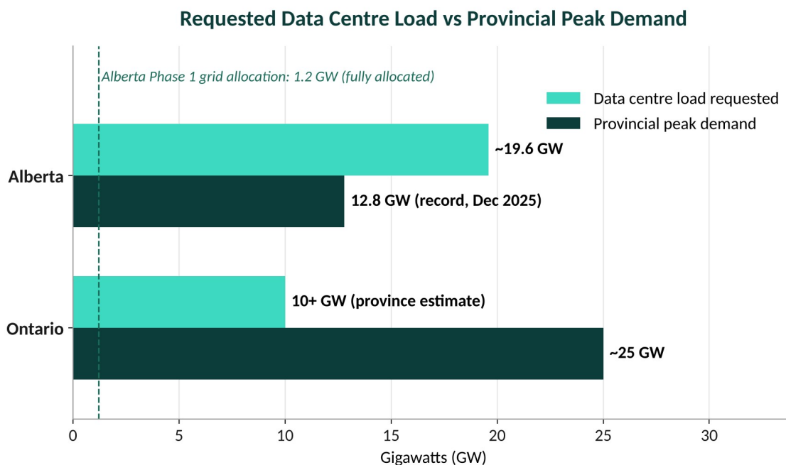
Exhibit 2. Requested data-centre load versus provincial peak demand, GW. Requested load covers all data-centre projects; the AI share is not separately reported. Sources: Government of Alberta (AESO connection list, July 30, 2026; record peak, December 11, 2025); Ontario Ministry of Energy and Mines via Dentons and Power Advisory (August–September 2026).
