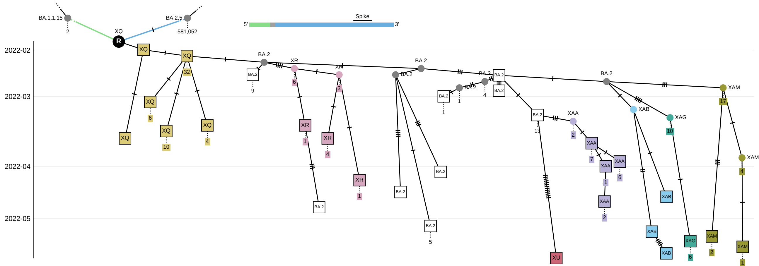
B Nested origin: XQ, XR, XU, XAA, XAB, XAG and XAM
