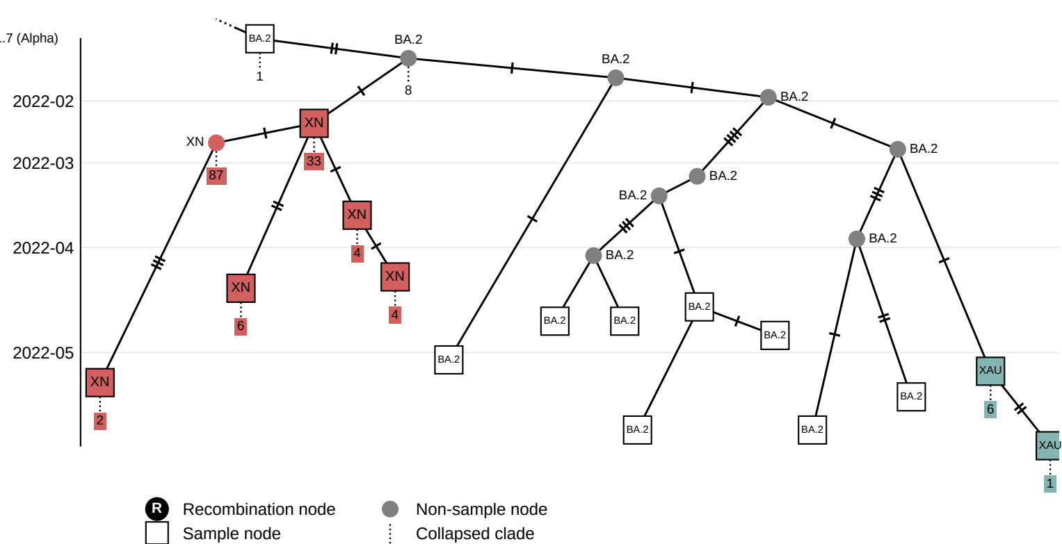
C Putative non-recombinants: XN and XAU
