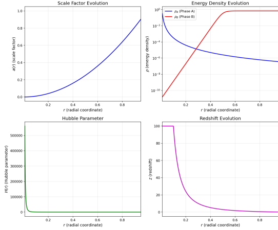
(a) Background energy density evolution.
