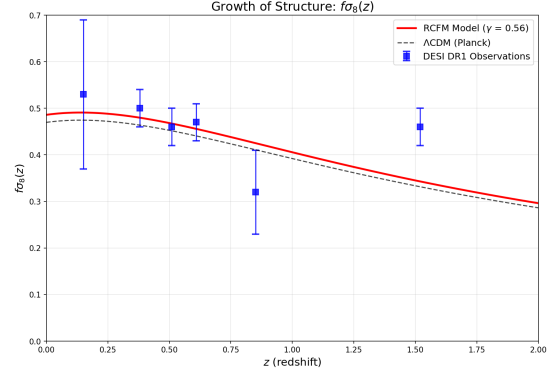
(a) f\sigma_8 constraints.
