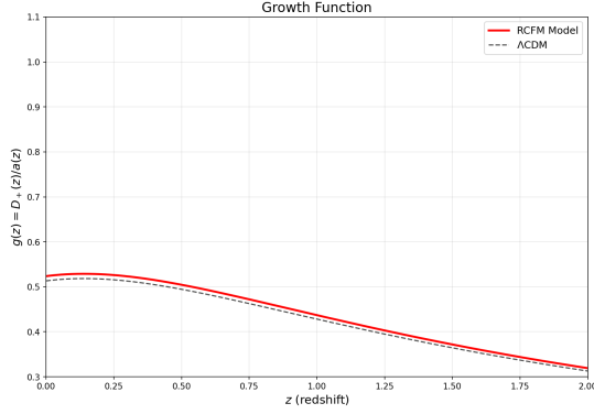
(b) Growth function g(z) .
