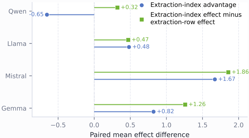
A Paired attribution differences
