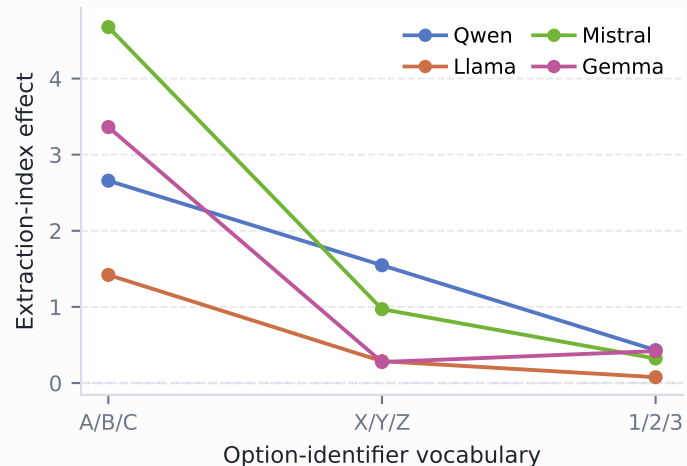
B Identifier-vocabulary sensitivity
