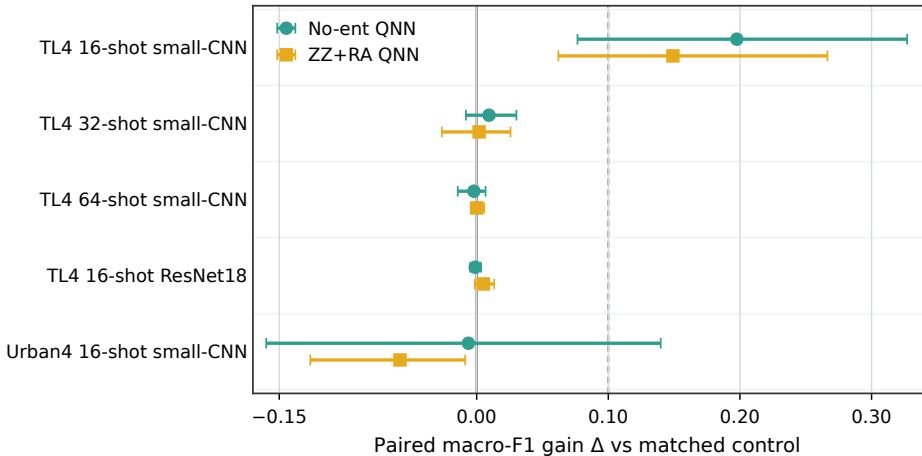
(a) Regime-level paired gains
