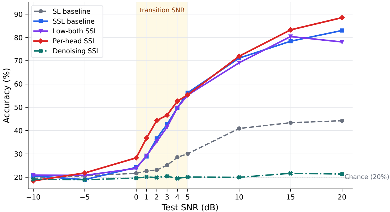
Dense SNR evaluation, label ratio 0.005
