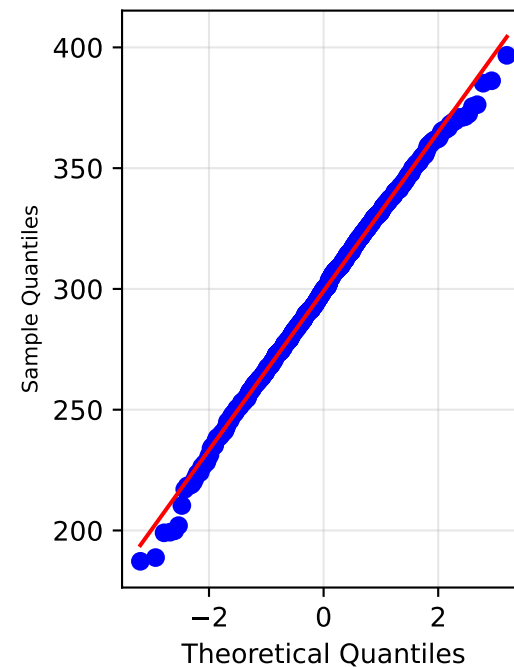
f_w Q-Q Plot
