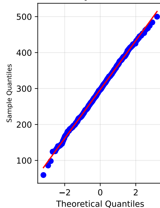
f_{avg} Q-Q Plot
