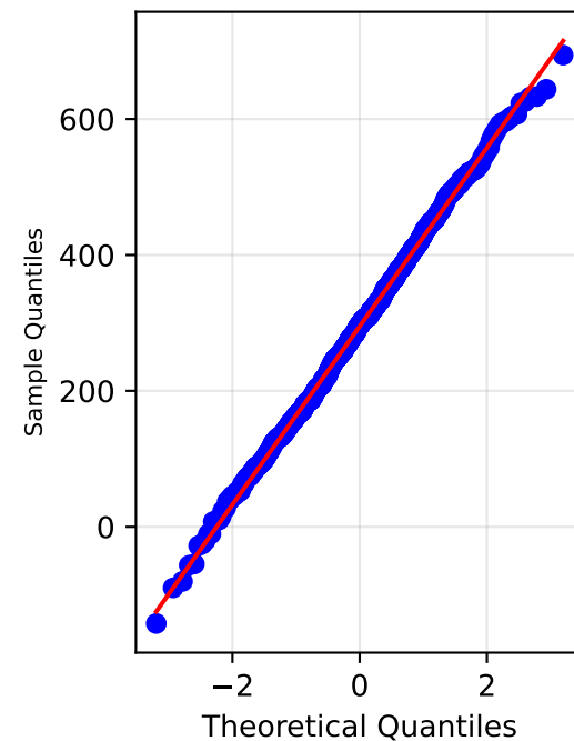
f_u Q-Q Plot
