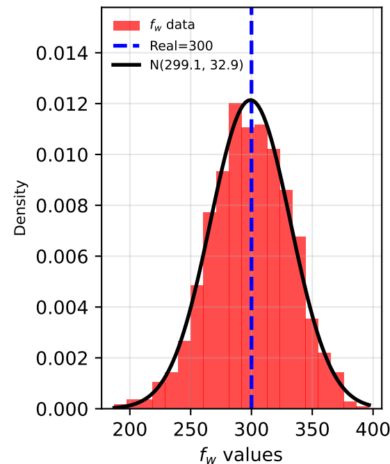
f_w (deg=334, Jarque-Bera score=0.137)
