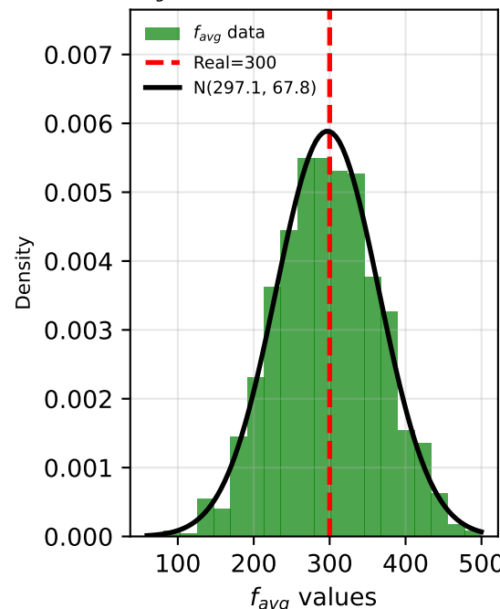
f_{avg} (Jarque-Bera score=0.570)
