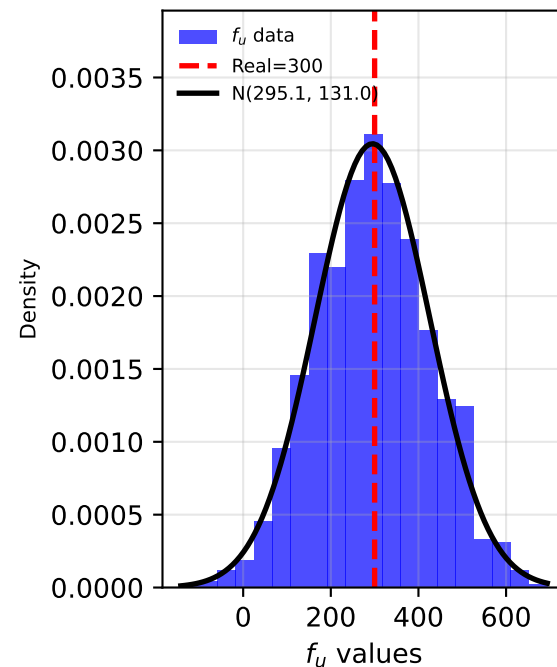
f_u (deg=5903, Jarque-Bera score=0.508)
