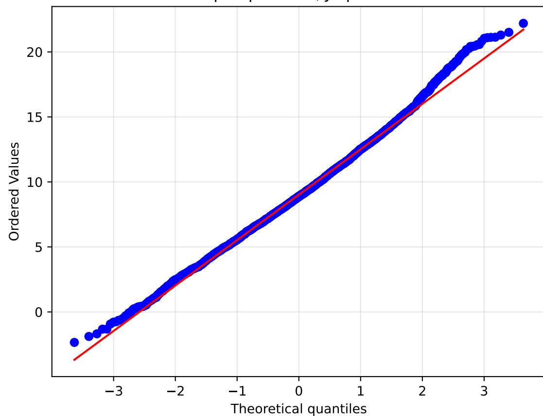
q=5: Skew=0.237, Kurt=0.012 Shapiro p=0.018, JB p=0.000
