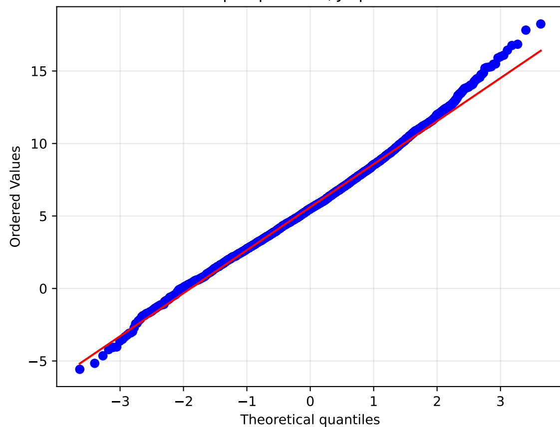
q=4: Skew=0.187, Kurt=0.037 Shapiro p=0.010, JB p=0.000
