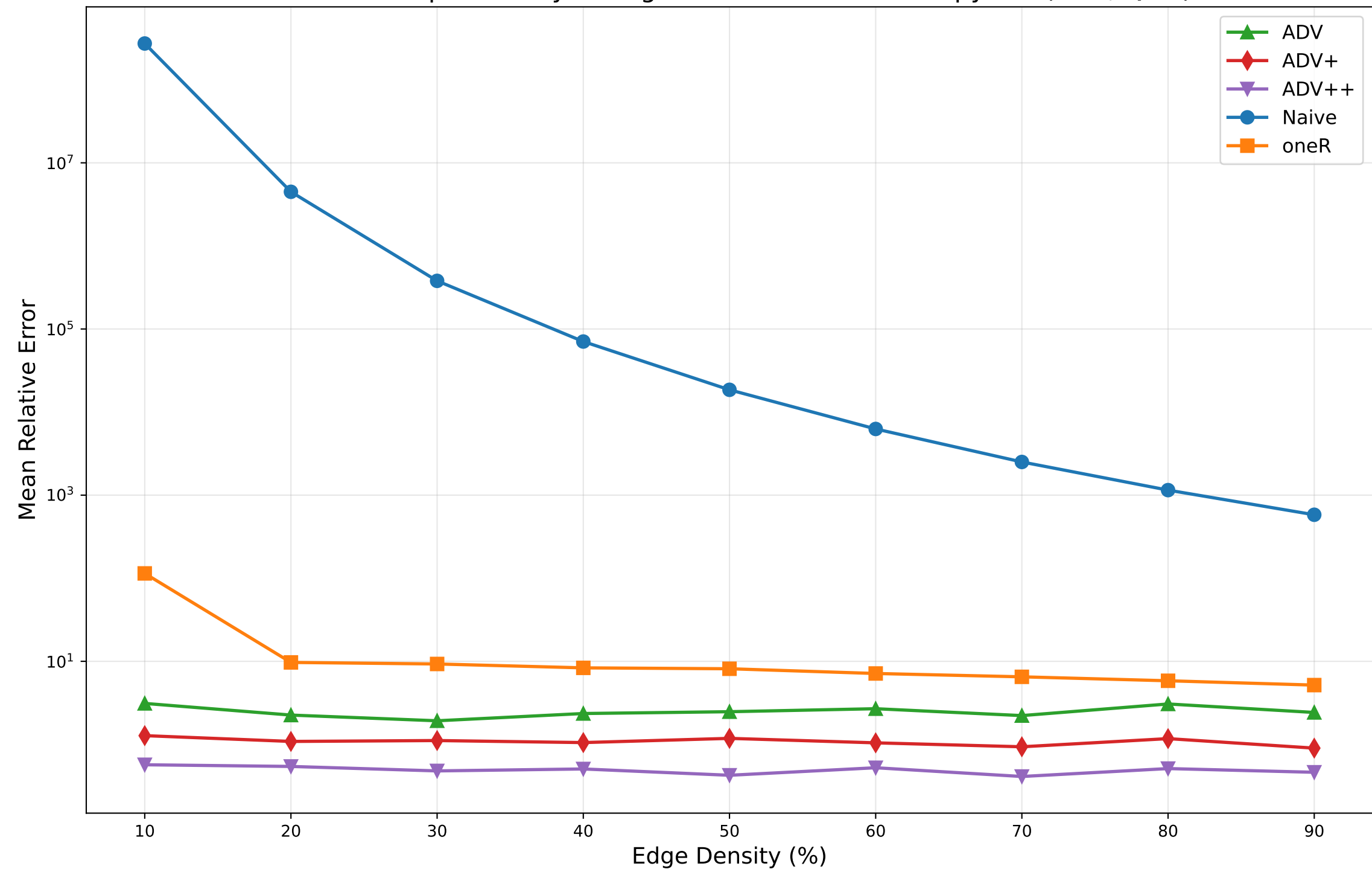
Effect of Graph Density on Algorithm Performance\nnbpywiki (P=2, Q=3)
