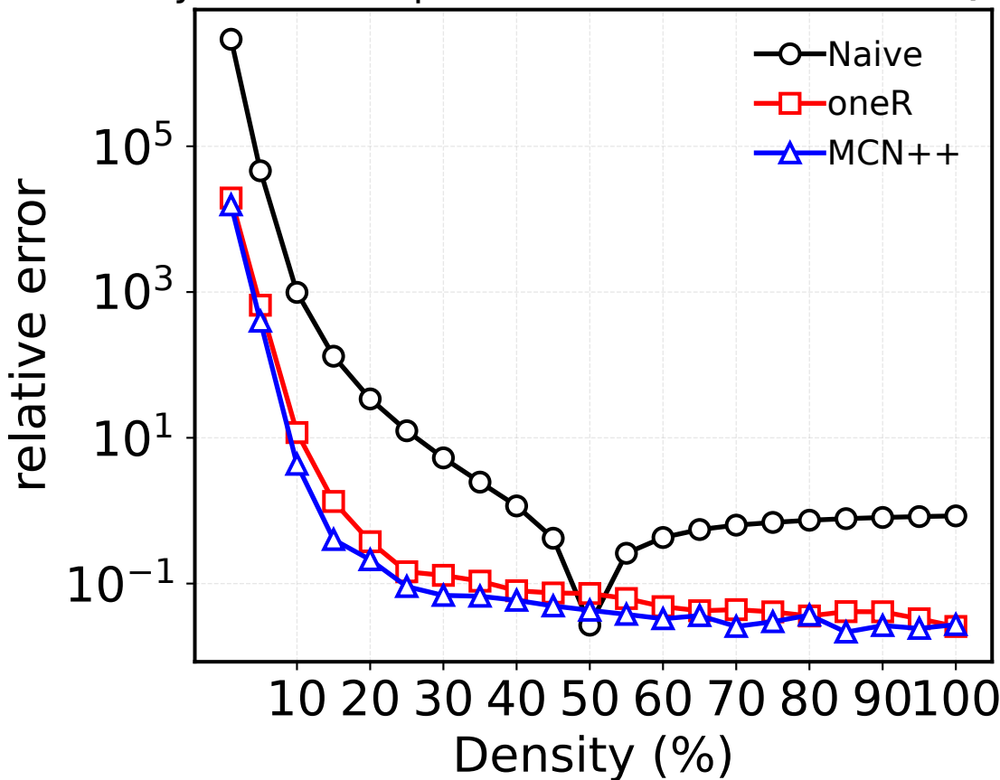
Synthetic Graph, n_1=100 , n_2=200 , P=2 , Q=3
