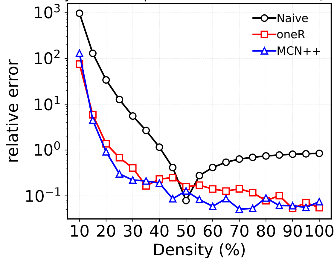
Synthetic Graph, n_1=50 , n_2=100 , P=2 , Q=3
