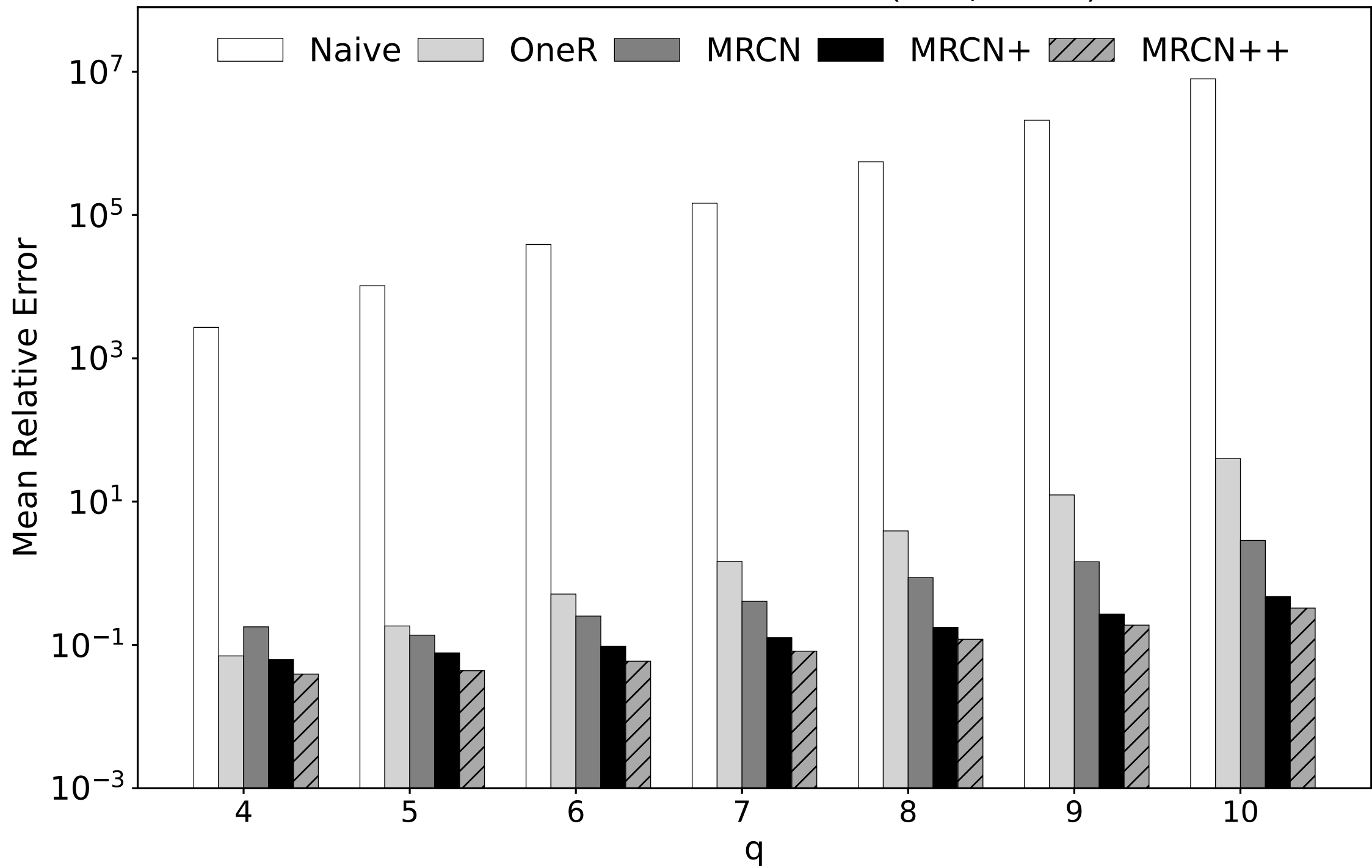
LIBREC-FILMTRUST-RATINGS Dataset ( P=2 , \epsilon=1.0 ) - FIXED
