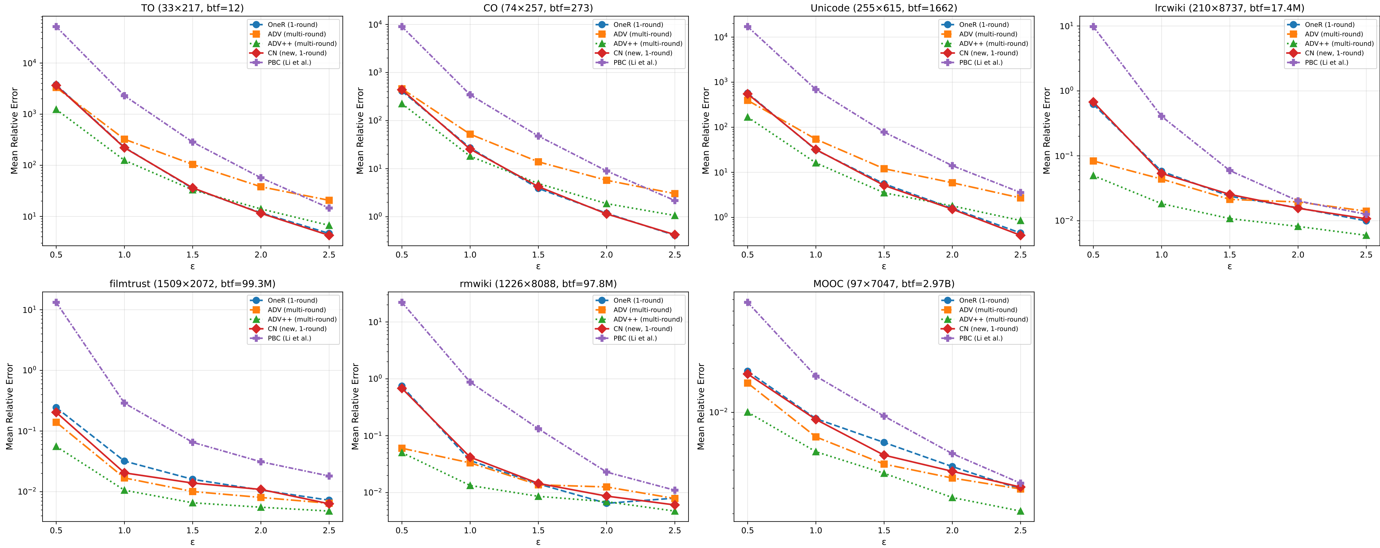
Algorithm Comparison: MRE vs \epsilon for (2,2)-Biclique Counting
