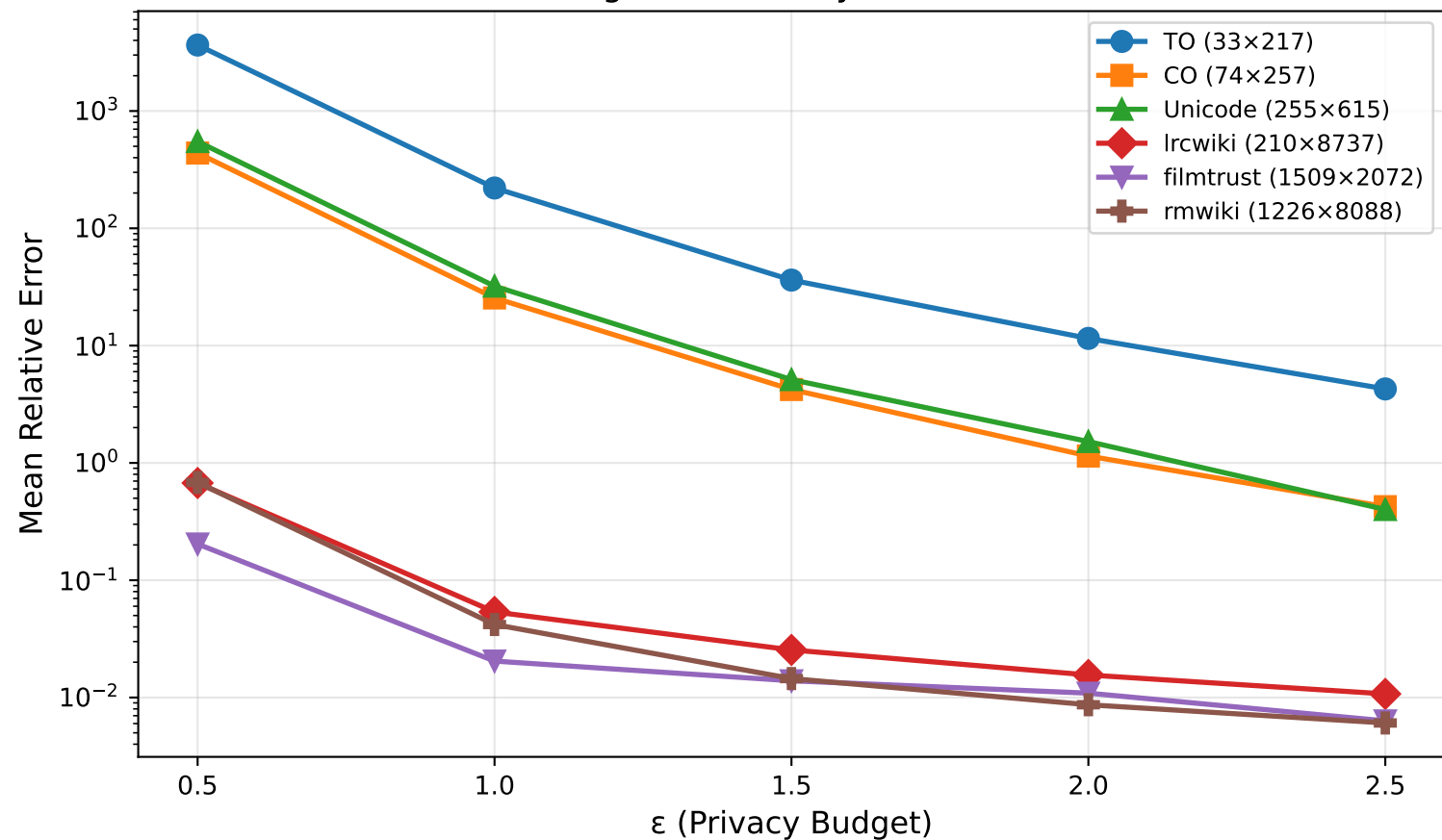
Common-Neighbor Butterfly Estimator: MRE vs \epsilon
