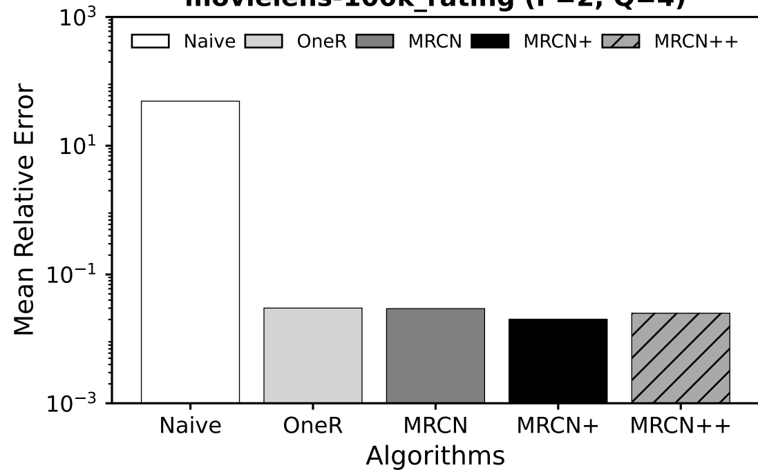
movielens-100k_rating (P=2, Q=4)
