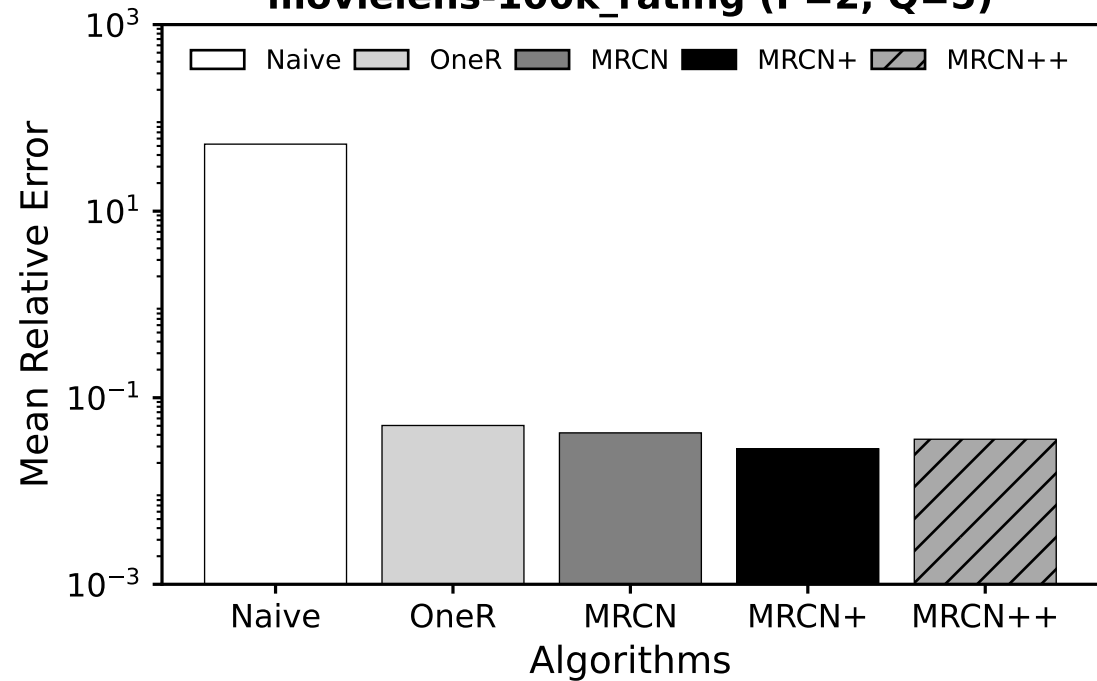
movielens-100k_rating (P=2, Q=5)
