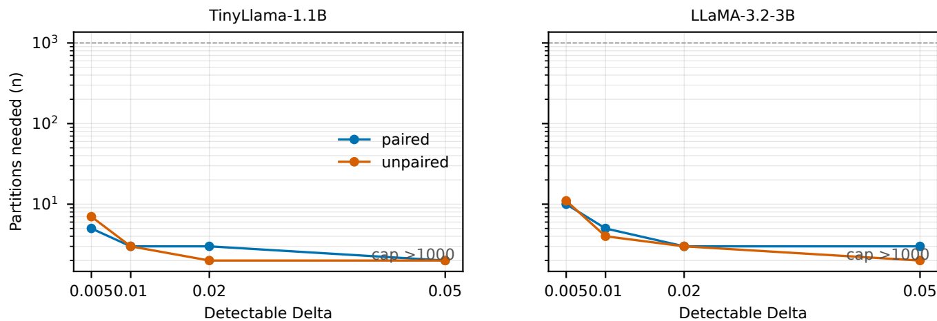
Fig. 3. Partition draws needed for pre-registered deltas and observed gaps.
