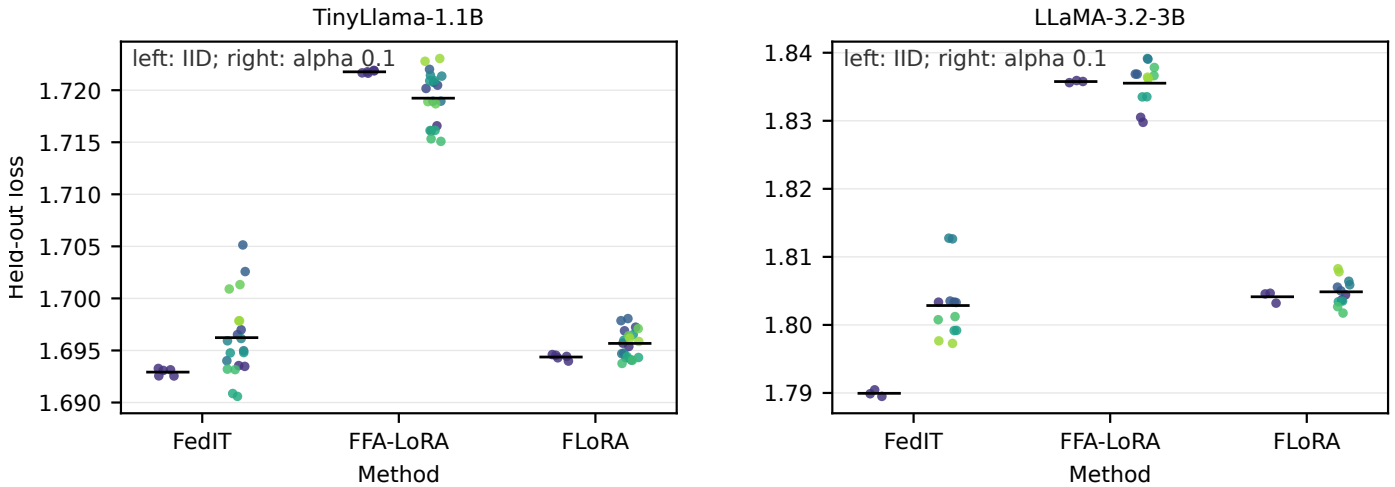
Fig. 1. Held-out loss by method and partition at Dirichlet \alpha=0.1 .
