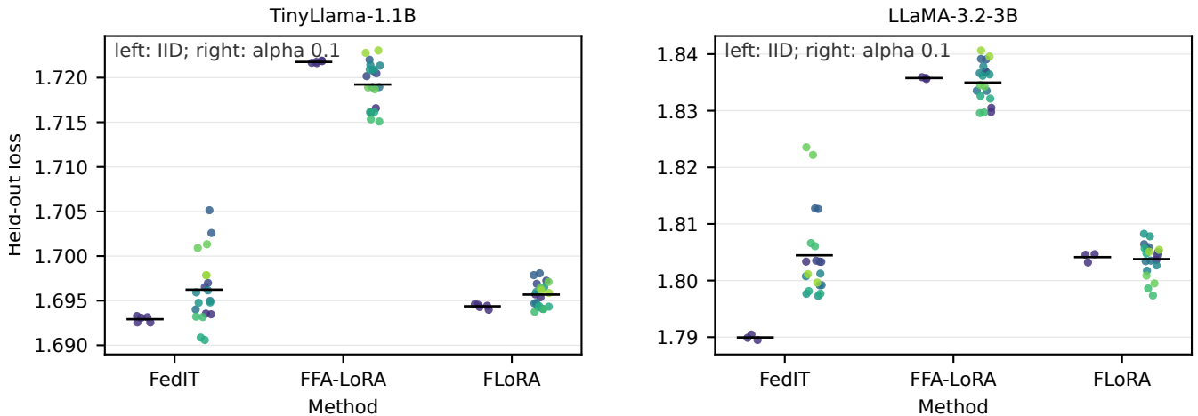
FIGURE 1. Held-out loss by method: IID (left group) and Dirichlet \alpha=0.1 (right group), points colored by partition.
