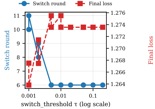
Fig. 3 ReverseAdaptive threshold sensitivity (TinyLlama IID, seed 42, MPS corpus). Communication is backend-invariant; loss values are not comparable with the CUDA results in Table 2
