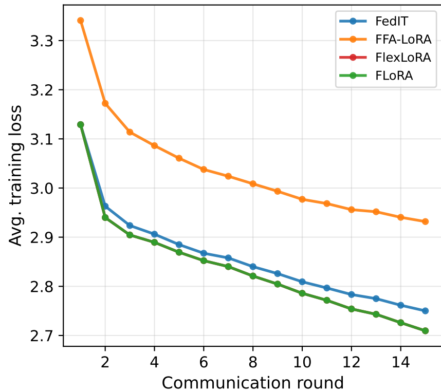
Label skew (CommonsenseQA)
