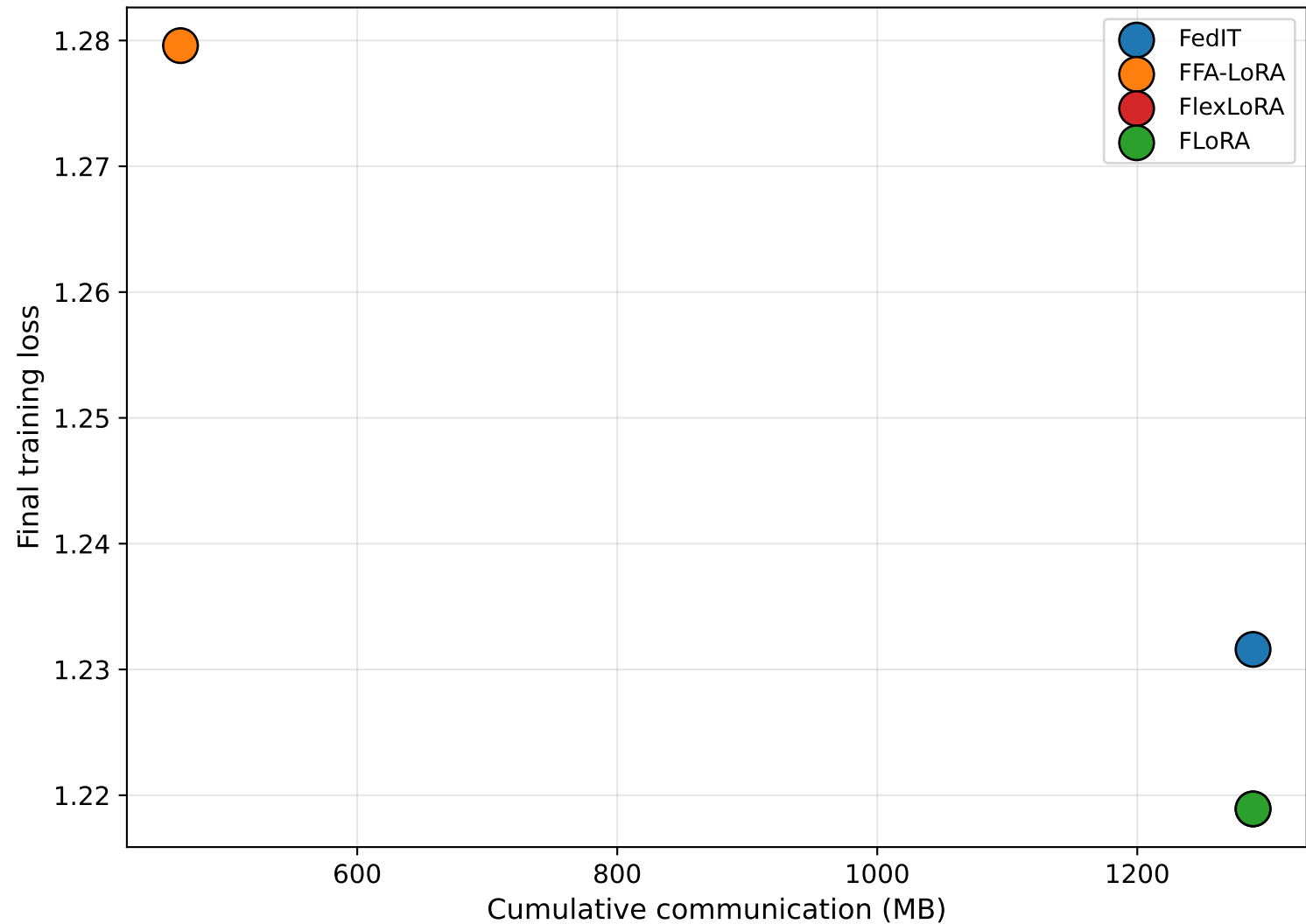
Communication vs loss (IID baseline, RQ3)
