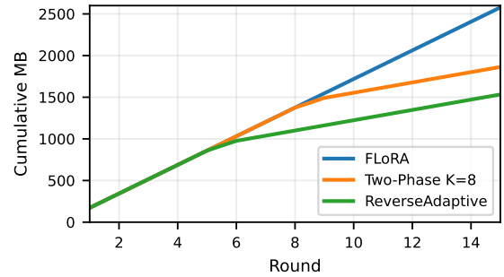
Fig. 3 Cumulative communication on TinyLlama-1.1B (seed 42, deterministic across seeds). Slope changes mark phase transitions: ReverseAdaptive at round 6, Two-Phase K=8 at round 9. The look-ahead download accounting causes the broadcast slope to change one round before the upload slope changes
