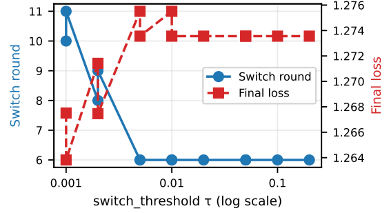
Fig. 4 ReverseAdaptive threshold sensitivity (TinyLlama IID, seed 42, MPS corpus). Communication is backend-invariant; loss values are not comparable with the CUDA results in Table 2
