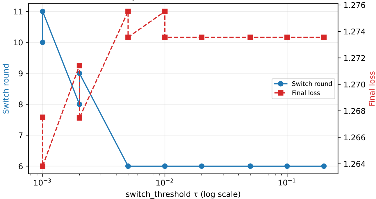
ReverseAdaptive threshold ablation (seed 42)
