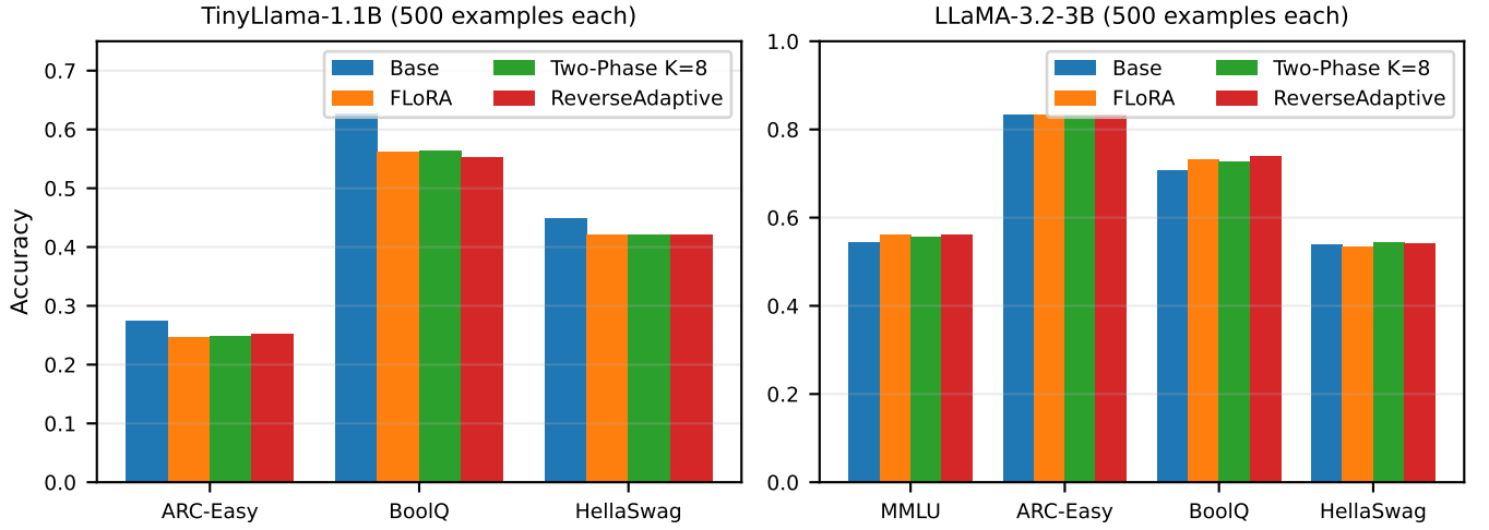
Fig. 1. Downstream zero-shot accuracy across two model scales (500 examples per benchmark). Left: TinyLlama-1.1B (seed 42 only; ARC-Easy, BoolQ, HellaSwag; MMLU omitted because base accuracy is at chance for 4-way multiple choice). Right: LLaMA-3.2-3B (mean across three seeds; MMLU, ARC-Easy, BoolQ, HellaSwag). Federated methods cluster within 1.0 percentage points at TinyLlama-1.1B, across the three informative benchmarks, and 0.5 percentage points at LLaMA-3.2-3B. TinyLlama accuracies are single-seed and from the MPS corpus; loss values elsewhere in the main paper for the same configurations are three-seed and from the CUDA corpus.
