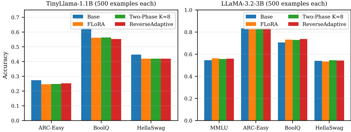
Fig. F1 Downstream zero-shot accuracies of Tables 4 and 5, restated graphically with no additional measurements (500 examples per benchmark). Left: TinyLlama-1.1B (seed 42 only; ARC-Easy, BoolQ, HellaSwag; MMLU omitted because base accuracy is at chance for 4-way multiple choice). Right: LLaMA-3.2-3B (mean across three seeds; MMLU, ARC-Easy, BoolQ, HellaSwag). Federated methods cluster within 1.0 percentage points at TinyLlama-1.1B, across the three informative benchmarks, and 0.5 percentage points at LLaMA-3.2-3B. TinyLlama accuracies are single-seed and from the MPS corpus; loss values elsewhere in this paper for the same configurations are three-seed and from the CUDA corpus
