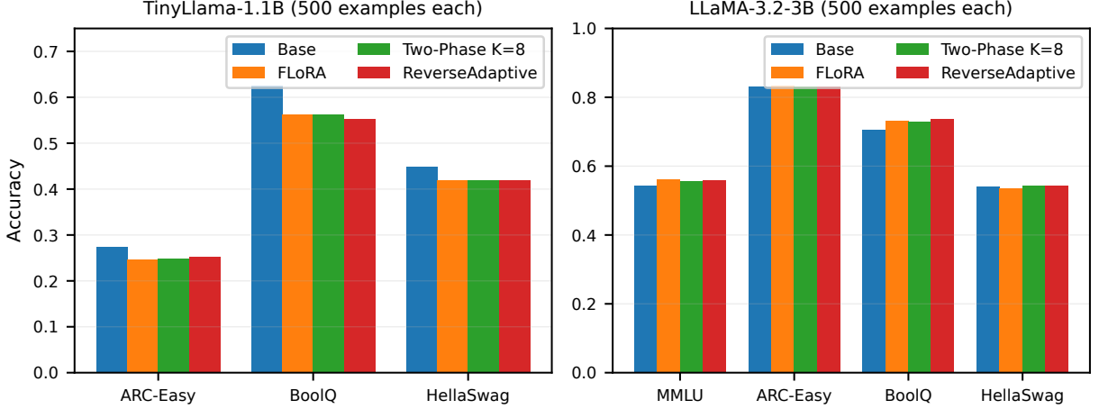
Fig. F1 Downstream zero-shot accuracy across two model scales (500 examples per benchmark). Left: TinyLlama-1.1B (seed 42 only; ARC-Easy, BoolQ, HellaSwag; MMLU omitted because base accuracy is at chance for 4-way multiple choice). Right: LLaMA-3.2-3B (mean across three seeds; MMLU, ARC-Easy, BoolQ, HellaSwag). Federated methods cluster within 1.0 percentage points at TinyLlama-1.1B, across the three informative benchmarks, and 0.5 percentage points at LLaMA-3.2-3B. TinyLlama accuracies are single-seed and from the MPS corpus; loss values elsewhere in this paper for the same configurations are three-seed and from the CUDA corpus
