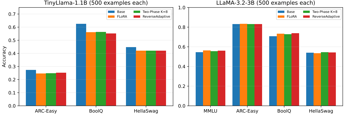
Fig. 4. Downstream zero-shot accuracy across two model scales (500 examples per benchmark). Left: TinyLlama-1.1B (seed 42 only; ARC-Easy, BoolQ, HellaSwag; MMLU omitted because base accuracy is at chance for 4-way multiple choice). Right: LLaMA-3.2-3B (mean across three seeds; MMLU, ARC-Easy, BoolQ, HellaSwag). Federated methods cluster within 1.0 percentage points at TinyLlama-1.1B, across the three informative benchmarks, and 0.5 percentage points at LLaMA-3.2-3B. TinyLlama accuracies are single-seed and from the MPS corpus; loss values elsewhere in this paper for the same configurations are three-seed and from the CUDA corpus.
