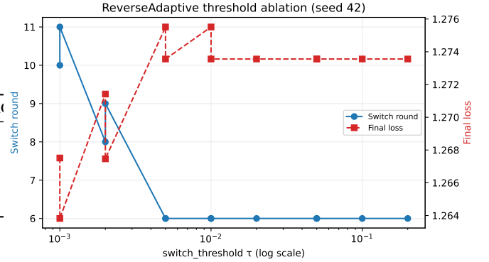
Fig. 5. ReverseAdaptive threshold sensitivity (TinyLlama IID, seed 42, MPS corpus). Communication is backend-invariant; loss values are not comparable with the CUDA results in Table II.
