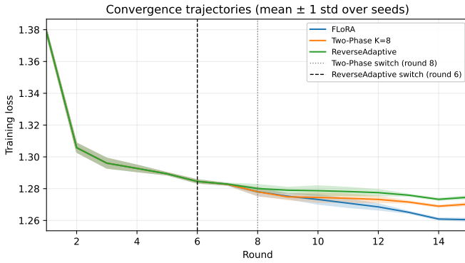
Fig. 2. Training loss trajectories on TinyLlama-1.1B IID. Mean \pm 1 standard deviation over three seeds. Vertical dashed lines mark ReverseAdaptive’s switch round (round 6) and Two-Phase K=8 ’s phase boundary (round 8); the transition round, in which the upload is still full, is round 9). All three methods converge similarly through the FLoRA phase; the loss gap accumulates gradually after the switch.
