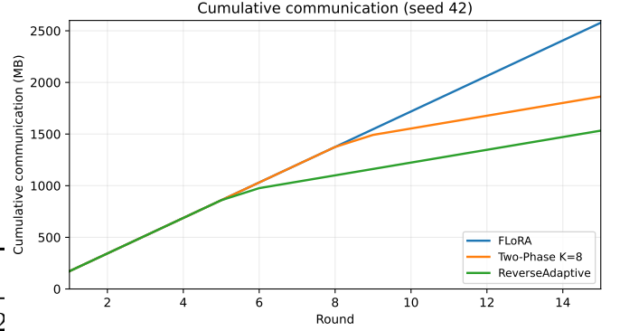
Fig. 3. Cumulative communication on TinyLlama-1.1B (seed 42, non-stochastic across seeds). Slope changes mark phase transitions: ReverseAdaptive at round 6, Two-Phase K=8 at round 9. The look-ahead download accounting causes the broadcast slope to change one round before the upload slope changes.
