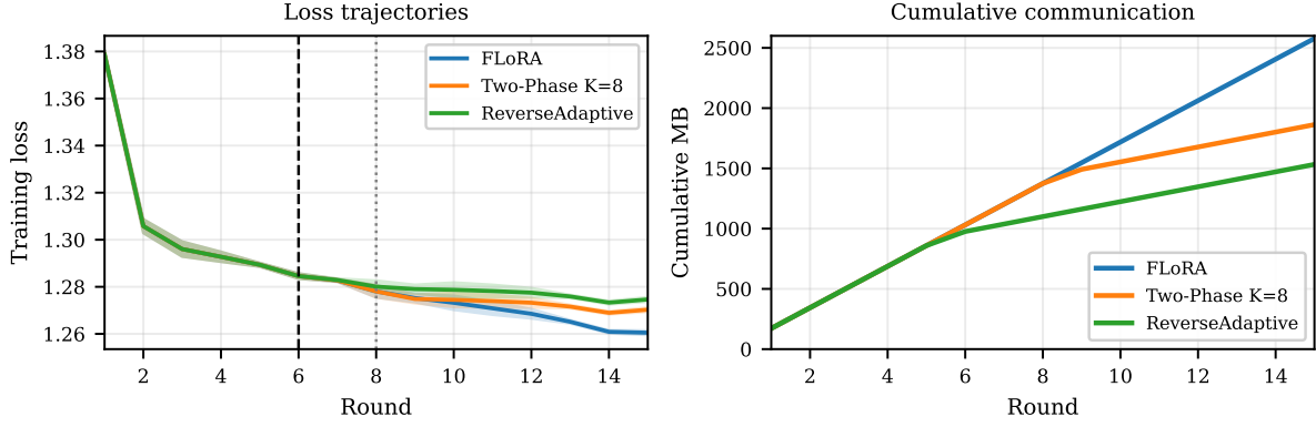
Fig. 2 Left: training loss trajectories on TinyLlama-1.1B IID, MPS corpus (mean \pm 1 standard deviation over three seeds). Vertical dashed lines mark ReverseAdaptive’s switch (round 6) and Two-Phase K=8 ’s phase boundary (round 8; the transition round, with full upload, is round 9). Right: cumulative communication on TinyLlama-1.1B (seed 42, deterministic across seeds). Slope changes mark phase transitions; look-ahead download accounting moves the broadcast slope one round before the upload slope
