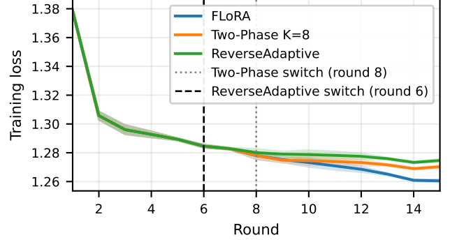
FIGURE 2. Training loss trajectories on TinyLlama-1.1B IID, MPS corpus. Mean \pm 1 standard deviation over three seeds. Per-round trajectories were logged on the MPS corpus; final-round values elsewhere in this paper are from CUDA. Vertical dashed lines mark ReverseAdaptive’s switch round (round 6) and Two-Phase K=8 ’s phase boundary (round 8; the transition round, in which the upload is still full, is round 9). All three methods converge similarly through the FLoRA phase; the loss gap accumulates gradually after the switch.
