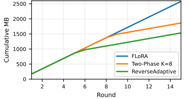
FIGURE 3. Cumulative communication on TinyLlama-1.1B (seed 42, deterministic across seeds). Slope changes mark phase transitions: ReverseAdaptive at round 6, Two-Phase K=8 at round 9. The look-ahead download accounting causes the broadcast slope to change one round before the upload slope changes.
