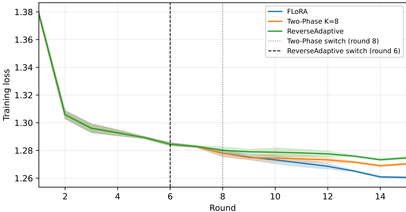
Convergence trajectories (mean \pm 1 std over seeds)
