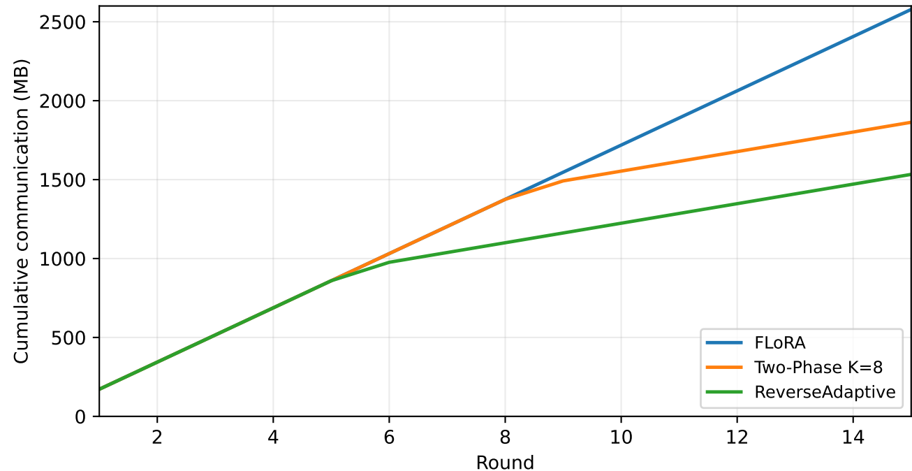
Cumulative communication (seed 42)
