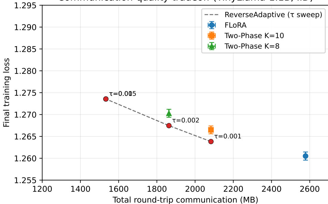
Communication-quality tradeoff (TinyLlama-1.1B, IID)
