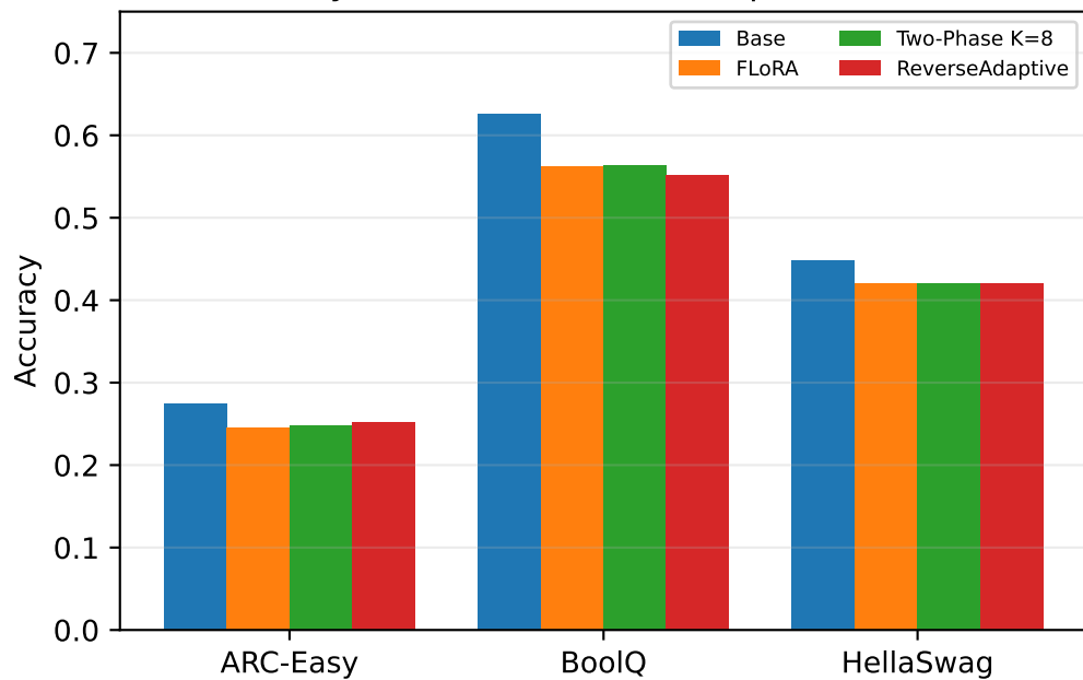
TinyLlama-1.1B (500 examples each)
