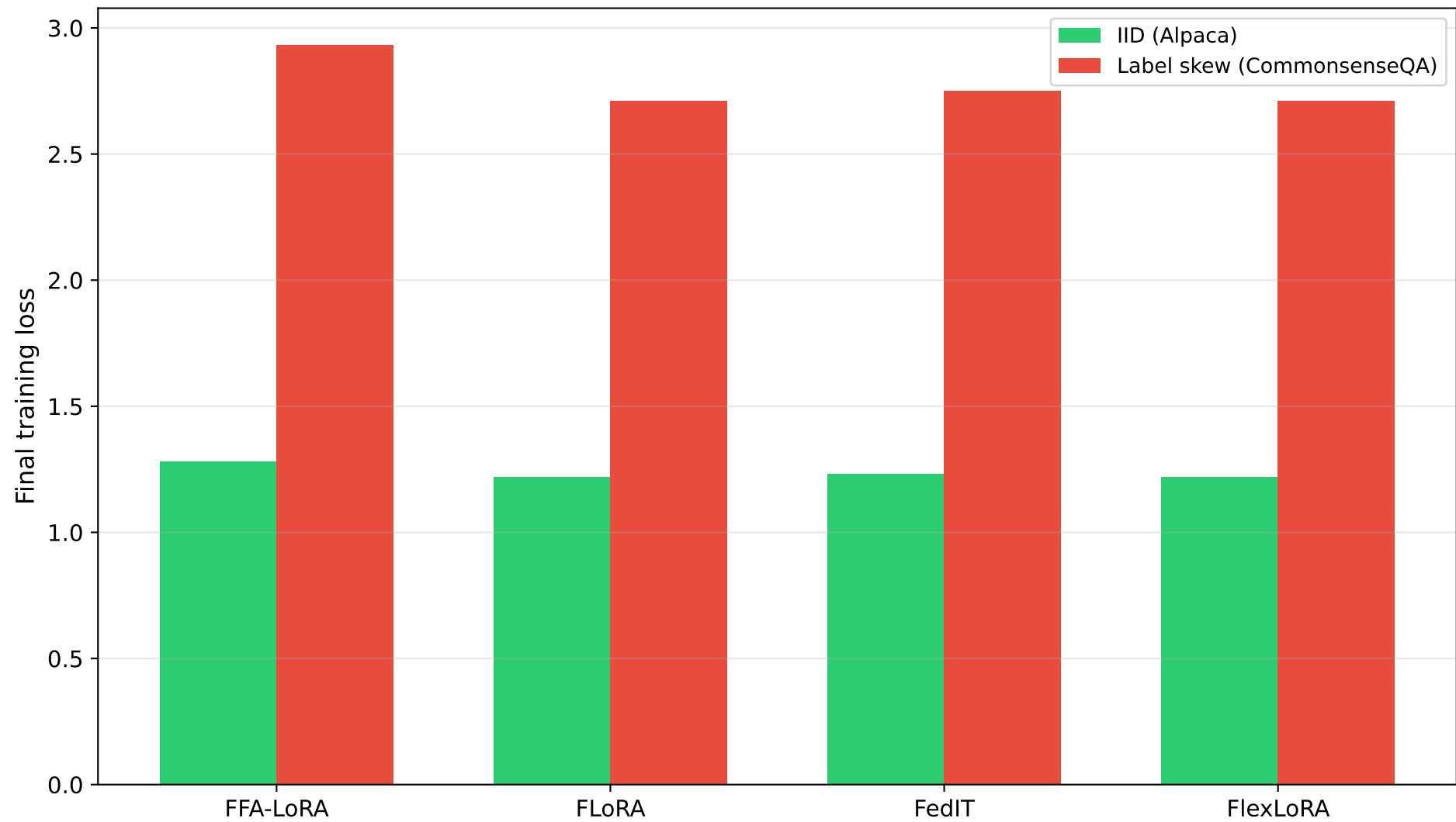
IID vs label-skew non-IID (final loss)
