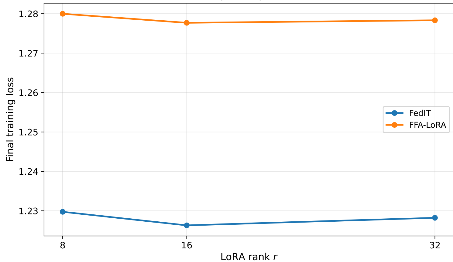
Rank sensitivity (IID Alpaca subset, RQ4)
