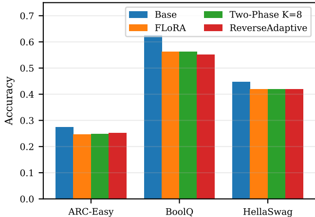
TinyLlama-1.1B (500 examples each)
