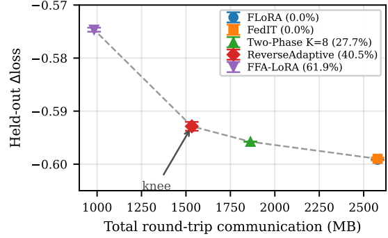
Fig. 1 Measured communication-quality frontier on Alpaca-3k, TinyLlama-1.1B, IID, CUDA corpus. Five protocols, three from prior work, at four distinct operating points; error bars are one sample standard deviation over three seeds, and communication is identical across seeds. Held-out \Delta\text{loss} is tuned minus base on the 500-example slice defined in Section 4.2; more negative is better. FLoRA and FedIT coincide at lower right. The segment from ReverseAdaptive to FFA-LoRA is markedly steeper than the segment preceding it, which Section 5.3 quantifies
