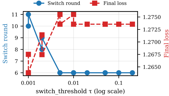
Fig. 3 ReverseAdaptive threshold sensitivity (TinyLlama IID, seed 42, MPS corpus). Communication is backend-invariant; loss values are not comparable with the CUDA results in Table 2
