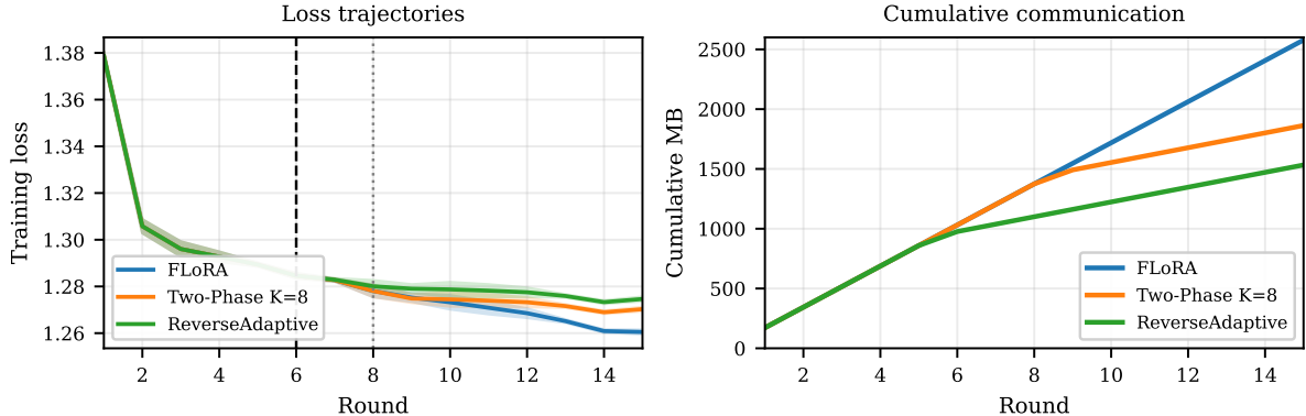
Fig. 2 Left: training loss trajectories on TinyLlama-1.1B IID, MPS corpus (mean \pm 1 standard deviation over three seeds). Vertical dashed lines mark ReverseAdaptive’s switch (round 6) and Two-Phase K=8 ’s phase boundary (round 8; the transition round, with full upload, is round 9). Right: cumulative communication on TinyLlama-1.1B (seed 42, deterministic across seeds). Slope changes mark phase transitions; look-ahead download accounting moves the broadcast slope one round before the upload slope
