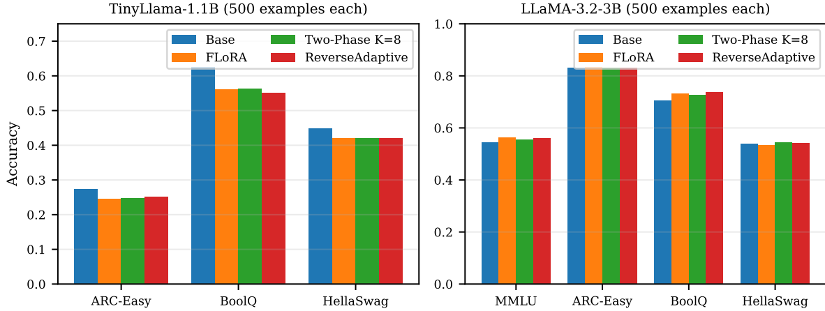
Fig. F1 Downstream zero-shot accuracy across two model scales (500 examples per benchmark). Left: TinyLlama-1.1B (seed 42 only; ARC-Easy, BoolQ, HellaSwag; MMLU omitted because base accuracy is at chance for 4-way multiple choice). Right: LLaMA-3.2-3B (mean across three seeds; MMLU, ARC-Easy, BoolQ, HellaSwag). Federated methods cluster within 1.0 percentage points at TinyLlama-1.1B, across the three informative benchmarks, and 0.5 percentage points at LLaMA-3.2-3B. TinyLlama accuracies are single-seed and from the MPS corpus; loss values elsewhere in this paper for the same configurations are three-seed and from the CUDA corpus
