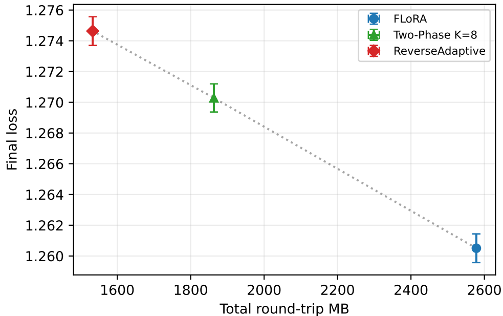
TinyLlama-1.1B (mean \pm 1 std, 3 seeds)
