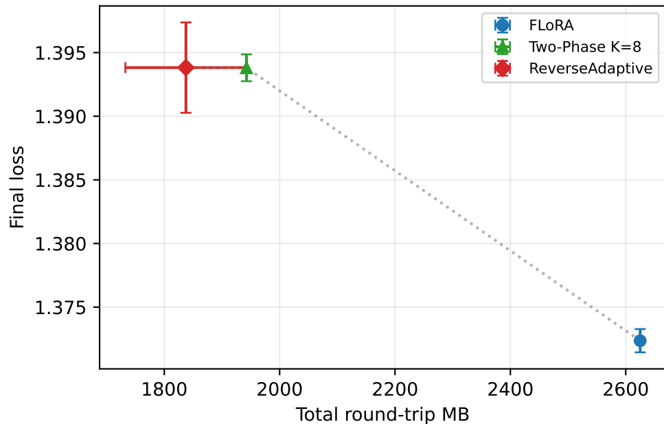
LLaMA-3.2-3B (mean \pm 1 std, 3 seeds)
