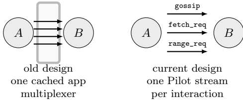
Figure 7: Current Pilot adapter stream lifecycle. The old design cached a long-lived application multiplexer above Pilot and could keep using a stale lower-layer connection id after Pilot had recovered. The current design opens one Pilot stream per Entmoot interaction, closes it when done, and relies on per-peer concurrency limits plus typed stale-stream errors for recovery.
