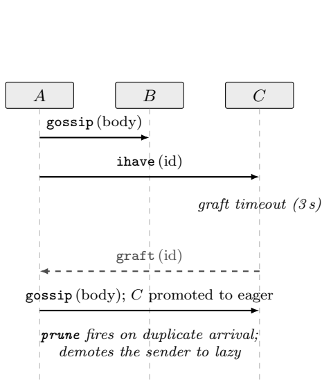
Figure 4: Plumtree spanning-tree repair. A eager-pushes the full message body to B and a lazy ihave advertisement to C . If the body has not arrived at C within 3 seconds, C sends graft to A , which replies with the body and promotes C back into its eager set. Symmetrically, a duplicate gossip frame triggers prune , demoting the redundant sender to lazy so subsequent messages arrive as ihave -only.
