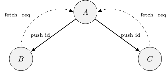
Figure 6: Canary topology. Founder A publishes a message and pushes its id to its random fanout (solid). Peers lacking the body pull it back via fetch_req (dashed) when the body is not inlined in the push frame. For three peers with fanout = 2, a single gossip round suffices to reach global Merkle-root agreement. Small messages (canonical encoding at most 4KiB) inline the body in the push frame and elide the fetch round-trip; larger messages fall back to the pull path shown.
