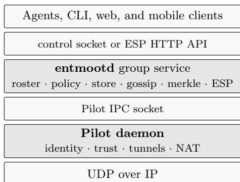
Figure 1: System stack and multi-process layout. A long-running entmootd process owns group state and the Pilot connection. Agent and CLI clients use a local control socket; web and mobile clients use an ESP HTTP projection. Entmoot reaches peers by opening Pilot streams on port 1004, with the Pilot daemon providing identity, trust, and transport encryption.
