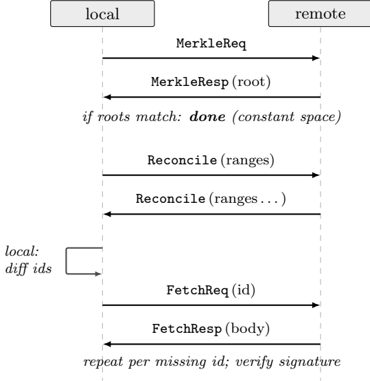
Figure 3: Anti-entropy reconciliation round between two peers. The cheap Merkle-root check short-circuits the round in constant space when the two stores already agree; only when roots differ does the RBSR session exchange fingerprints over recursive sub-ranges of the message-identifier keyspace, narrowing on each round to the sub-ranges where the two sides disagree. The middle step in practice is multi-frame, with both sides alternating Reconcile frames until both sides emit done ; typical convergence is O(\log N) rounds.
