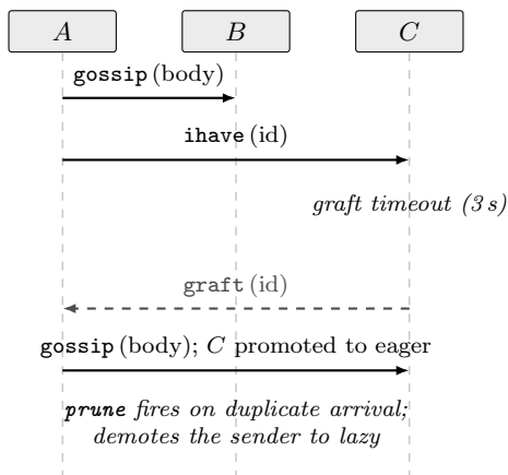
Figure 2: Plumtree spanning-tree repair. A eager-pushes the full message body to B and a lazy ihave advertisement to C . If the body has not arrived at C within 3 seconds, C sends graft to A , which replies with the body and promotes C back into its eager set. Symmetrically, a duplicate gossip frame triggers prune , demoting the redundant sender to lazy so subsequent messages arrive as ihave -only.
