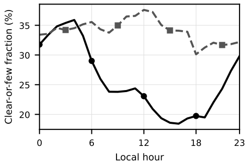
(b) Calgary: human vs. automated
