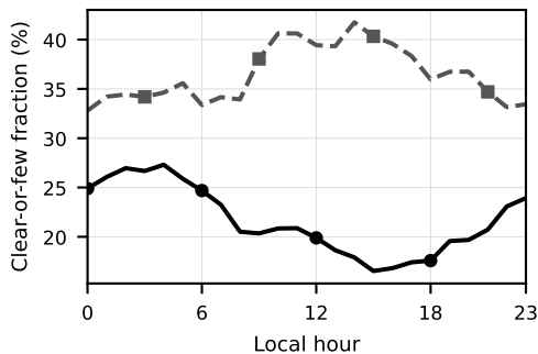
(e) Edmonton: human vs. automated
