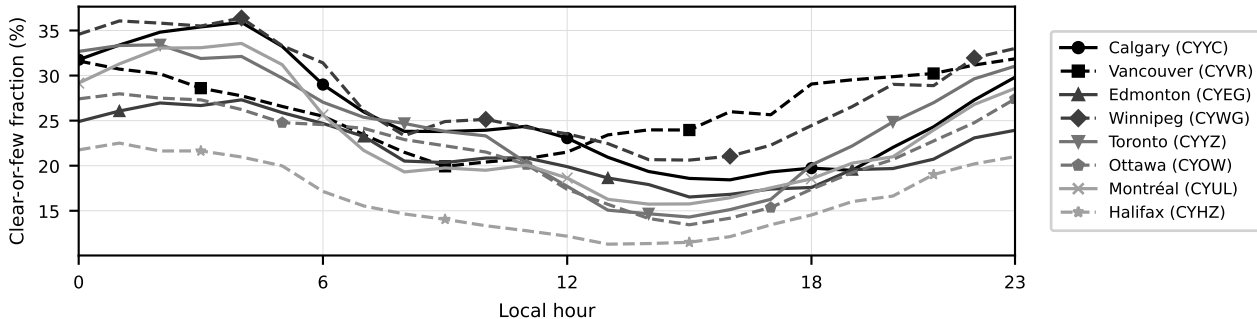
(a) Human METAR — all sites
