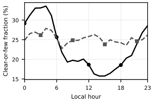
(c) Montréal: human vs. automated
