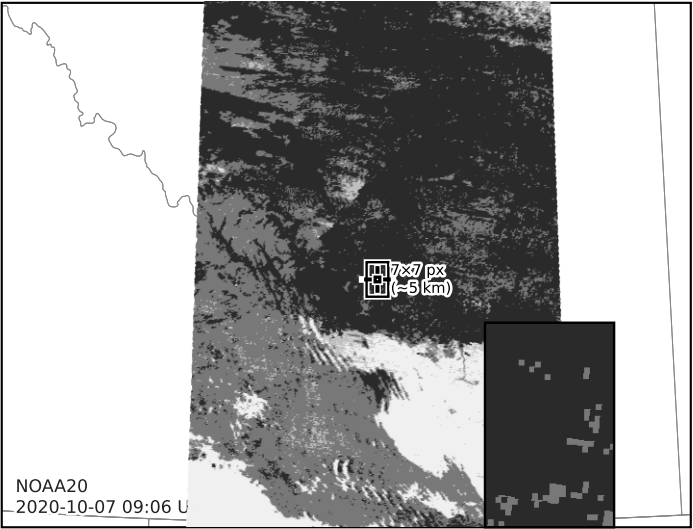
VIIRS MVCM (~750 m, near-nadir)
