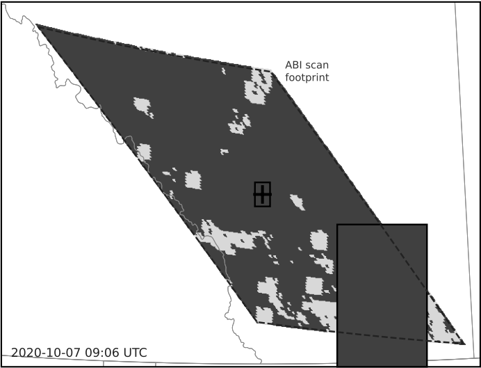
Cloud mask comparison: GOES ABI vs VIIRS MVCM — Calgary area GOES-East ABI BCM (~2 km, oblique ~69°)
