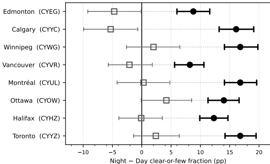
Human-augmented vs GOES satellite: night–day clear-sky bias All 8 cities. Human 2020–2025; GOES Enterprise mask, Dec 2021–2025. Dotted line = human – satellite difference
