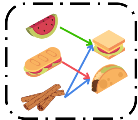
Causal relationships
