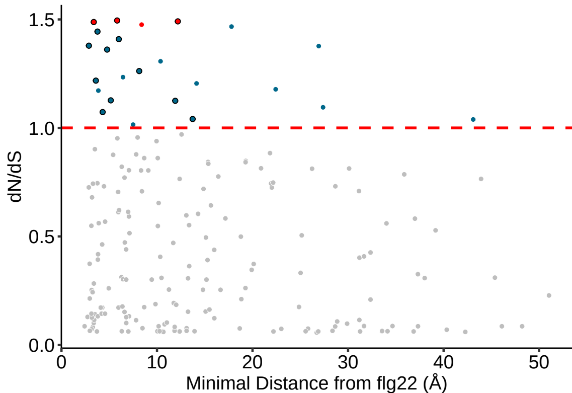
AtFLS2 Distance from flg22, all atoms
