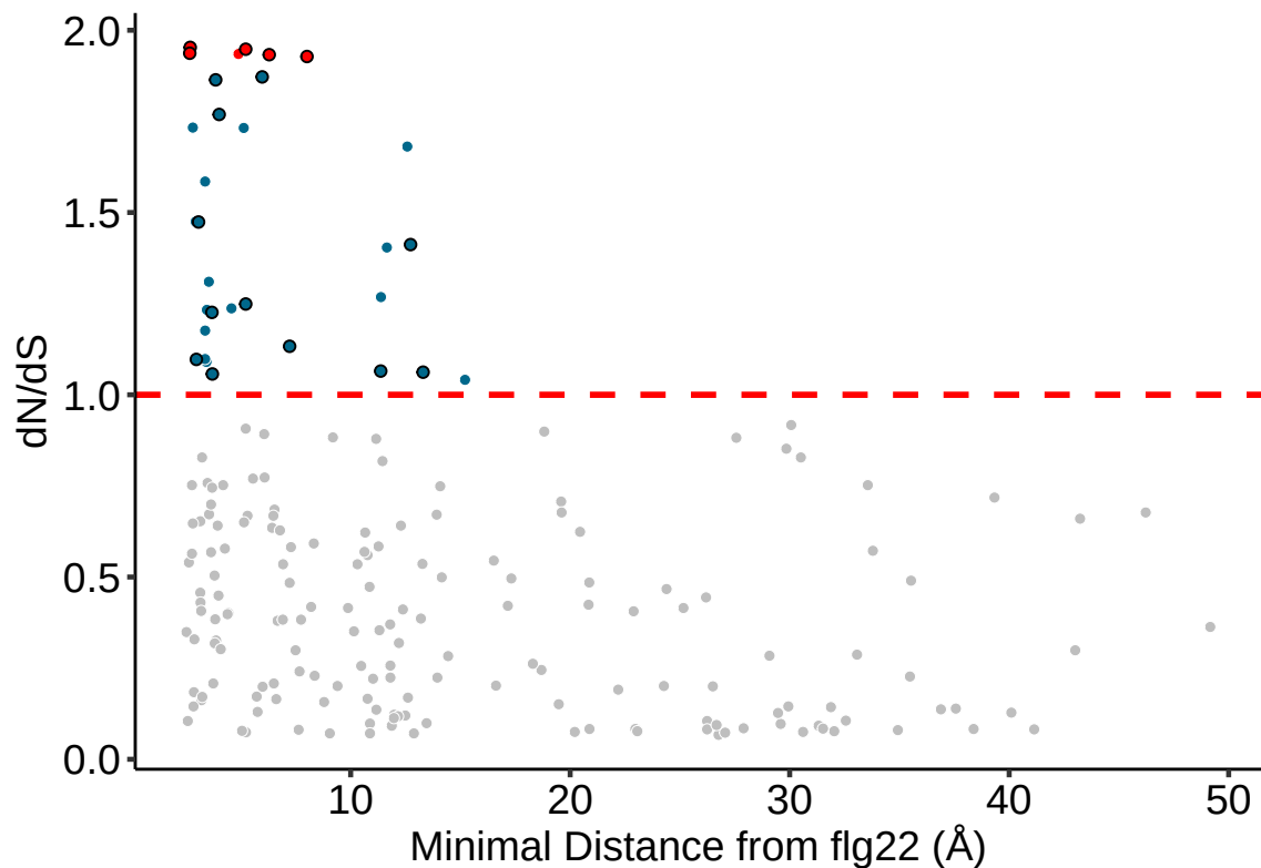
MdFLS2 Distance from flg22, all atoms
